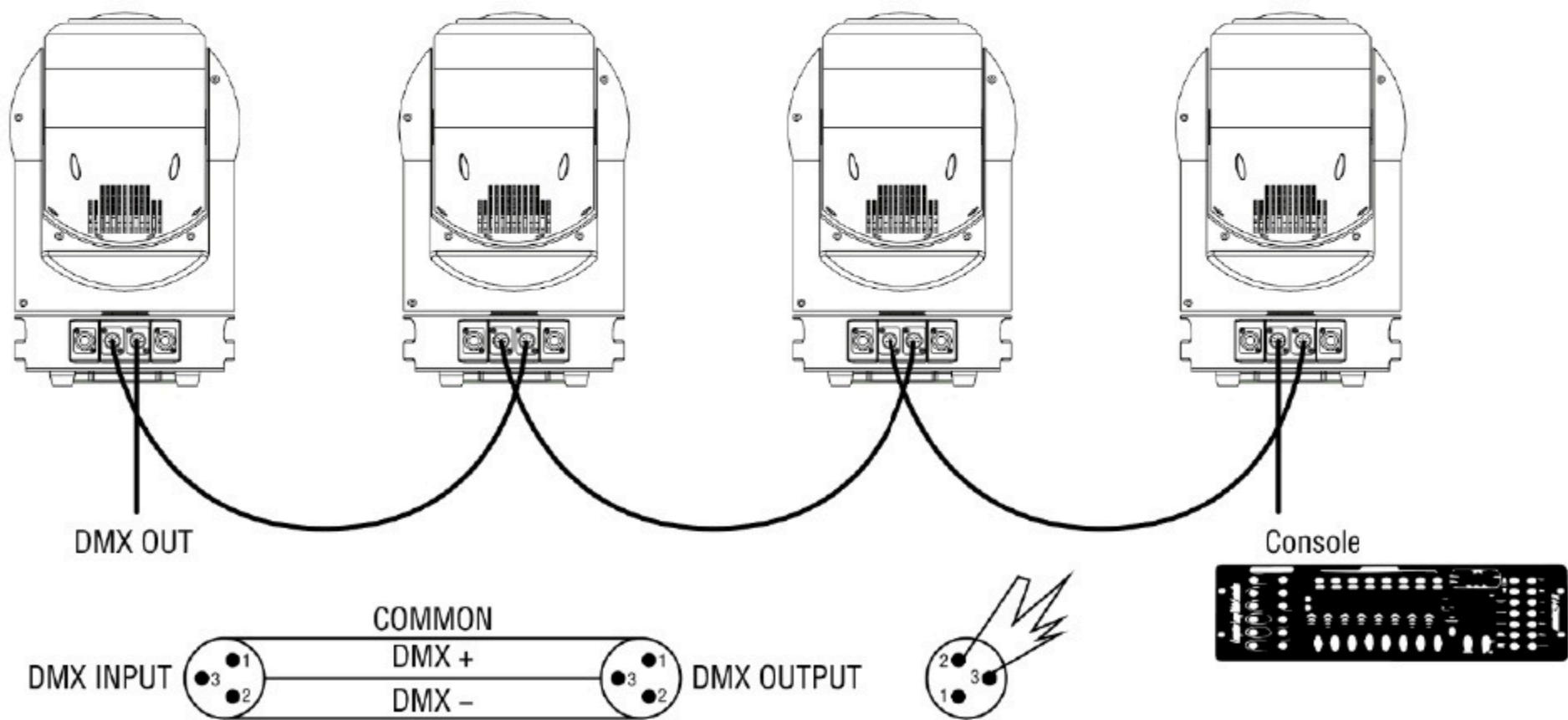
Figure 1 Schematic diagram of DMX signal wire connection
